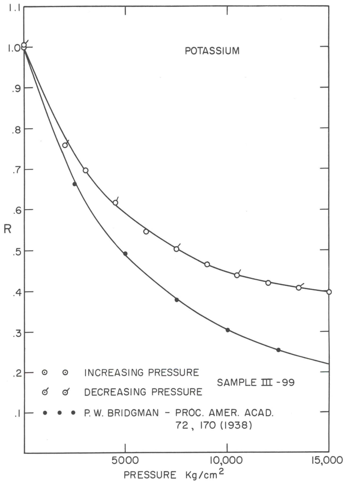
FIG. 3-6 NORMALIZED RESISTANCE R, vs. PRESSURE
